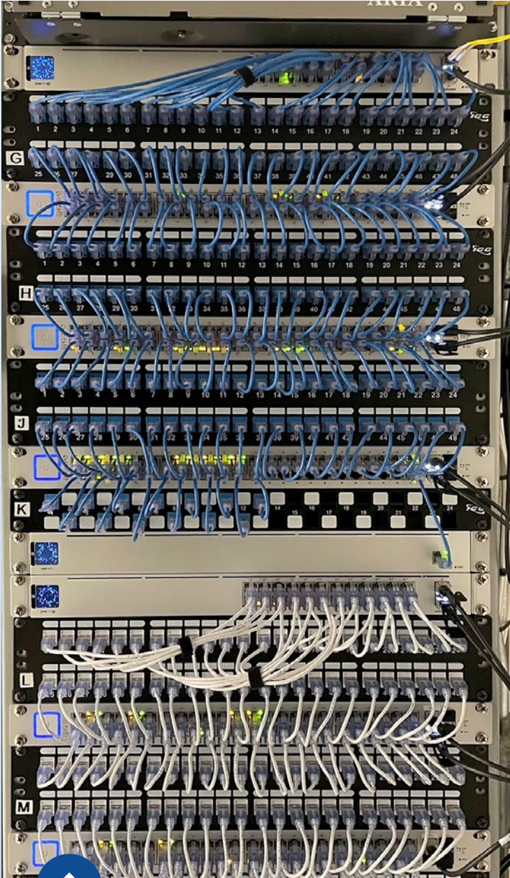
Front of voice and data rack with switches and patch cables designed for easy trouble shooting.
