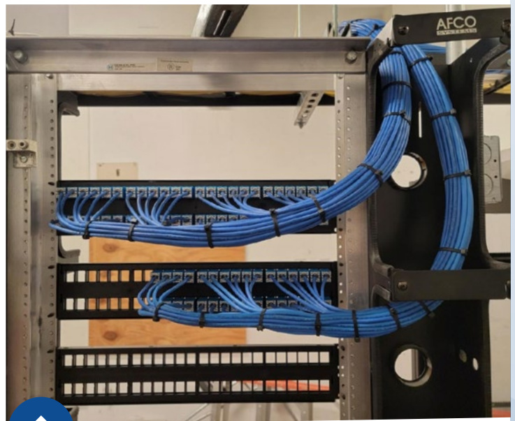
Orderly installation of data cabling integrated into the back of a patch panel.
